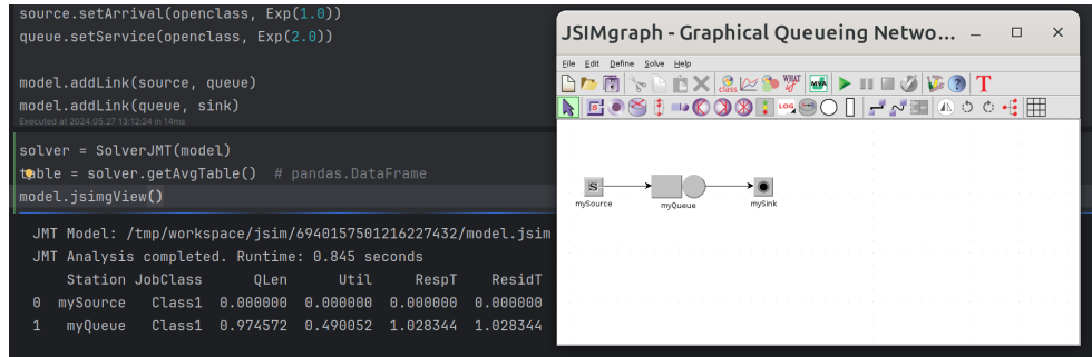
Figure 2.1: M/M/1 example in JSIMgraph launched from the DataSpell IDE
