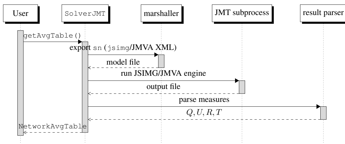
Figure 14.1: Sequence diagram of SolverJMT: marshal, run subprocess, parse.
