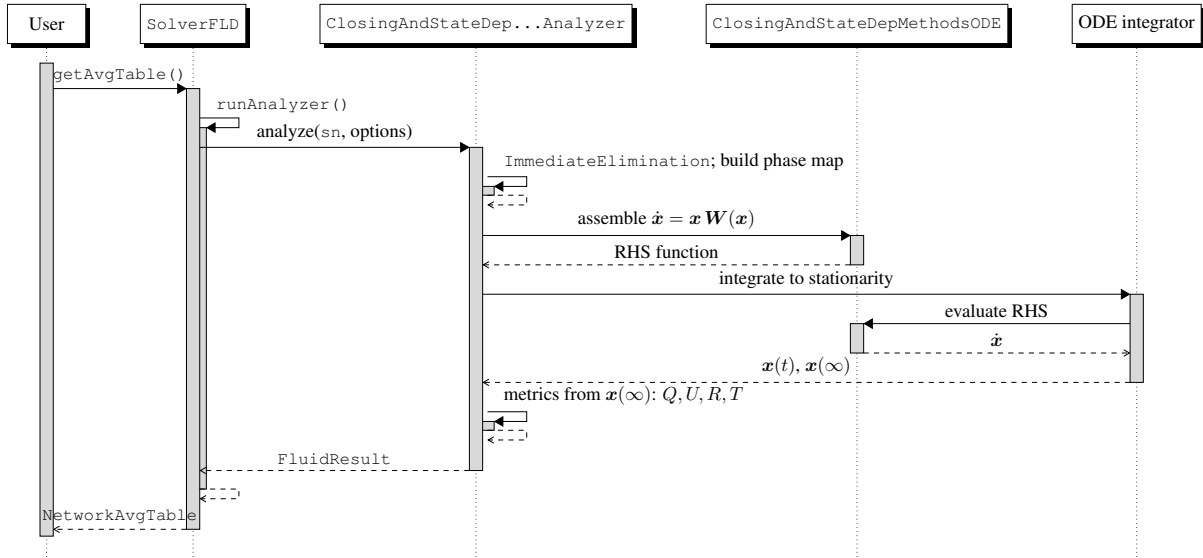
Figure 4.1: Sequence diagram of SolverFLD with the default closing method.
